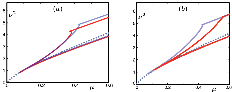
Figure 34. Comparison of the snaking region of localized hexagon patches (blue) and the snaking regions of planar \langle 10 \rangle hexagon pulses (red) in panel (a) and \langle 11 \rangle hexagon pulses (red) in panel (b). The hexagon Maxwell curve is also shown (dashed grey).
