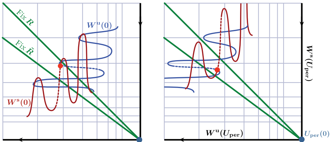
Figure 9. Shown is the dynamics of the linearized Poincaré map near the periodic orbit U_{\text{per}} . On the left, the parameter \mu is close to the pitchfork bifurcation in \text{Fix } \tilde{\mathcal{R}} that creates an asymmetric localized structure U_{\text{asym}}(0) (red bullet). As \mu is increased, we assume that W^u(0) is moved to the left and, correspondingly, by reversibility, W^s(0) is moved upward. Following their intersection U_{\text{asym}}(0) , which occurs along the branches plotted with dashes, we observe that it ends at a second pitchfork bifurcation in \text{Fix } \tilde{\mathcal{R}} . Thus, the asymmetric localized structures connect, in parameter space, even solutions with a minimum at x = 0 to even solutions with a maximum at x = 0 . The points U_{\text{asym}}(0) stay on the same horizontal and vertical segments of the invariant manifolds, and their distance from U_{\text{per}}(0) therefore does not change much: In particular, their L^2 -norm cannot change by too much, which explains why the ladders are approximately horizontal. See also the accompanying animation (70762_02.mov [533KB]).
