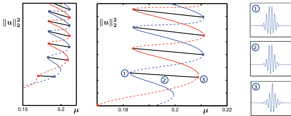
Figure 8. The left and center panels contain the bifurcation diagrams of asymmetric localized structures that bifurcate at pitchfork bifurcations from even localized structures [20, 22]: Solutions along the curved branches are even with minima (blue) or maxima (red) at x = 0 , while solutions along the horizontal ladders (black) are asymmetric. Panels 1–3 contain the graphs of selected solution profiles u(x) .
