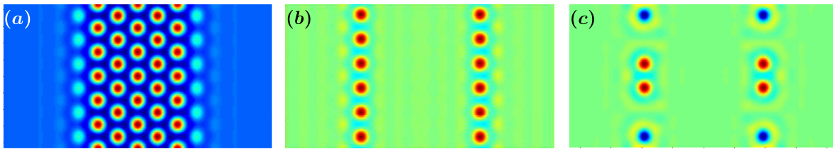
Figure 22. Shown are color plots of a planar \langle 10 \rangle hexagon pulse at a fold bifurcation in (a), the associated fold eigenfunction in (b), and the pitchfork eigenmode that leads to almost-planar hexagon pulses in (c).
