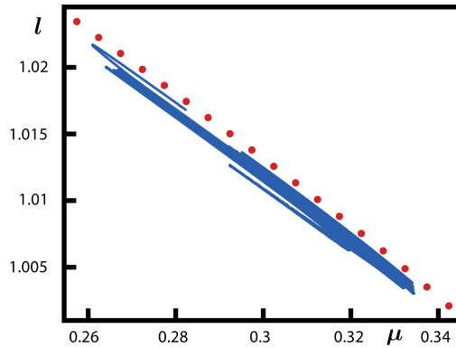
Figure 30. Plotted are the wavelengths l = 1/\kappa of the regular hexagons for which \mathcal{H} = 0 (red bullets) and of the hexagon cells located at the center of the localized hexagon patches (blue dots) as functions of \mu for \nu = 1.6 . The wavelength l = 1 corresponds to a spatial period of 2\pi .
