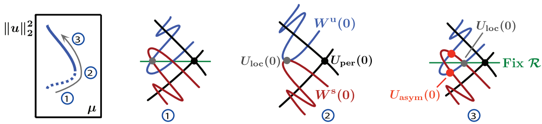
Figure 7. As we move upward on the snaking curve, \mu first increases and then decreases. Geometrically, the localized structure moves from one branch of the invariant manifolds through a saddle-node bifurcation to the adjacent branch. In doing so, it moves closer to the periodic orbit: Thus, it spends more “time” x near U_{\text{per}} and therefore broadens in space. As a result, its norm increases, which explains the structure of the snaking curve. Besides saddle-node bifurcations, the localized structures also undergo pitchfork bifurcations, which result in two asymmetric structures explained further in the text and in Figure 8.
