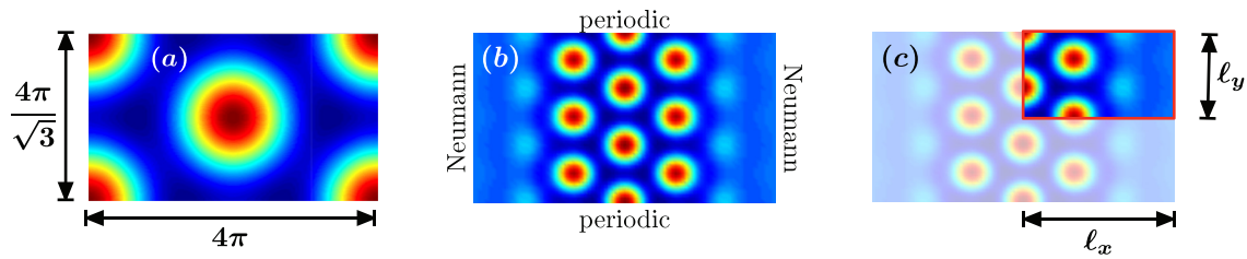
Figure 13. Regular hexagons are computed with Neumann boundary conditions on the domain \Omega_{\text{hex}} shown in panel (a). Reflection-symmetric planar hexagon pulses are defined on the domain shown in panel (b) with Neumann conditions in the horizontal x -direction and periodic boundary conditions in the vertical y -direction. Panel (c) illustrates the computational domain \Omega = (0, \ell_x) \times (0, \ell_y) with Neumann conditions.
